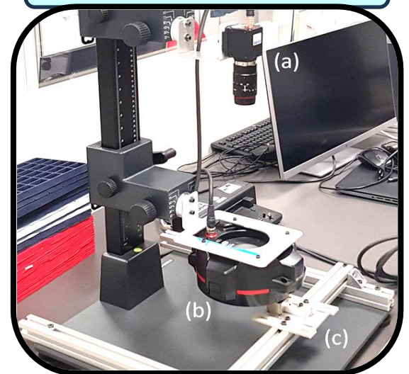
Vision System
