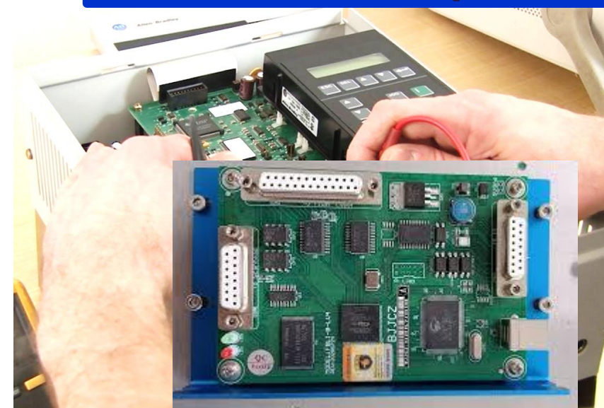
Siemens Drive/HMI
