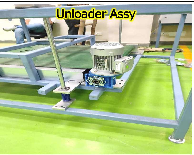
Conv Testing
