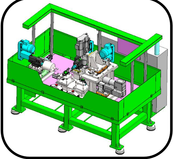
SPM Manufacturing
