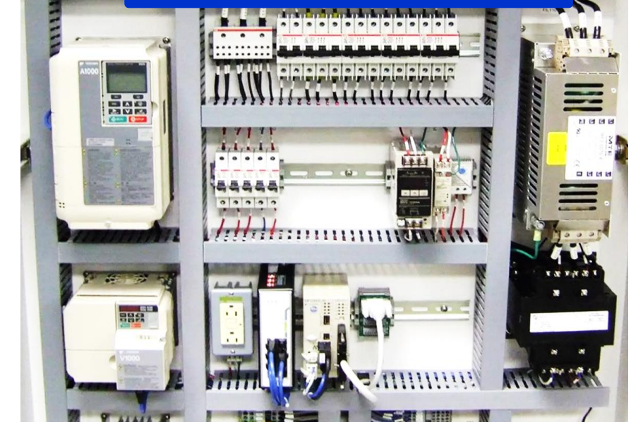
VFD Panel
