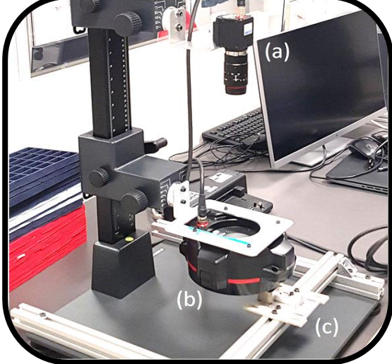
Vision System
